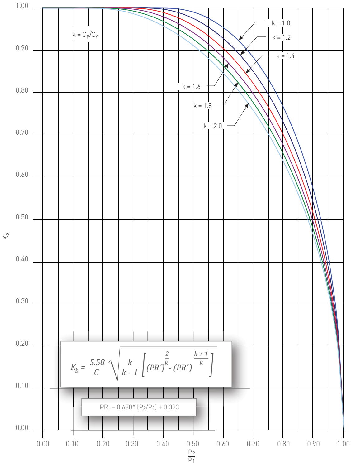
FIGURE 8-26 Anderson Greenwood Series LCP Pilot Operated PRV Back Pressure Correction Factor ( K_b ) - Gas Service
